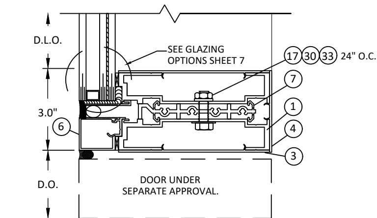
D 3 VERTICAL SECTION HORIZONTAL MULLION - DOOR HEAD CONNECTION - INSULATED GLASS
