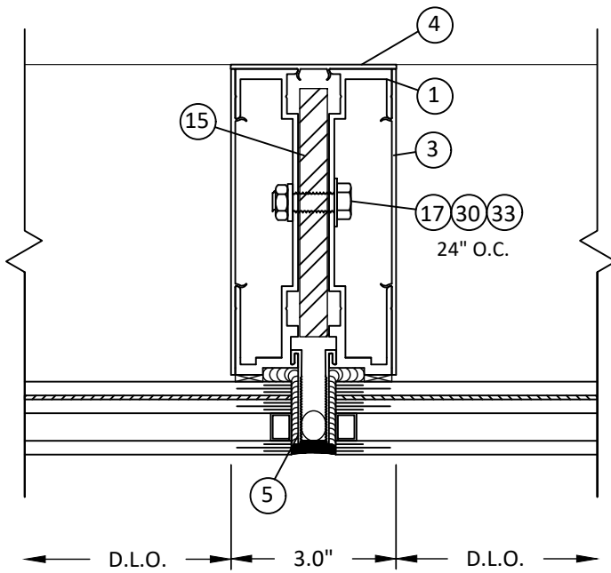
A 4 HORIZONTAL SECTION INTEGRATED VERTICAL INTERMEDIATE - INSULATED GLASS
