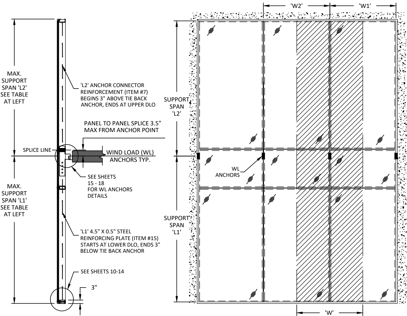
VERTICAL SECTION TWIN SPAN
