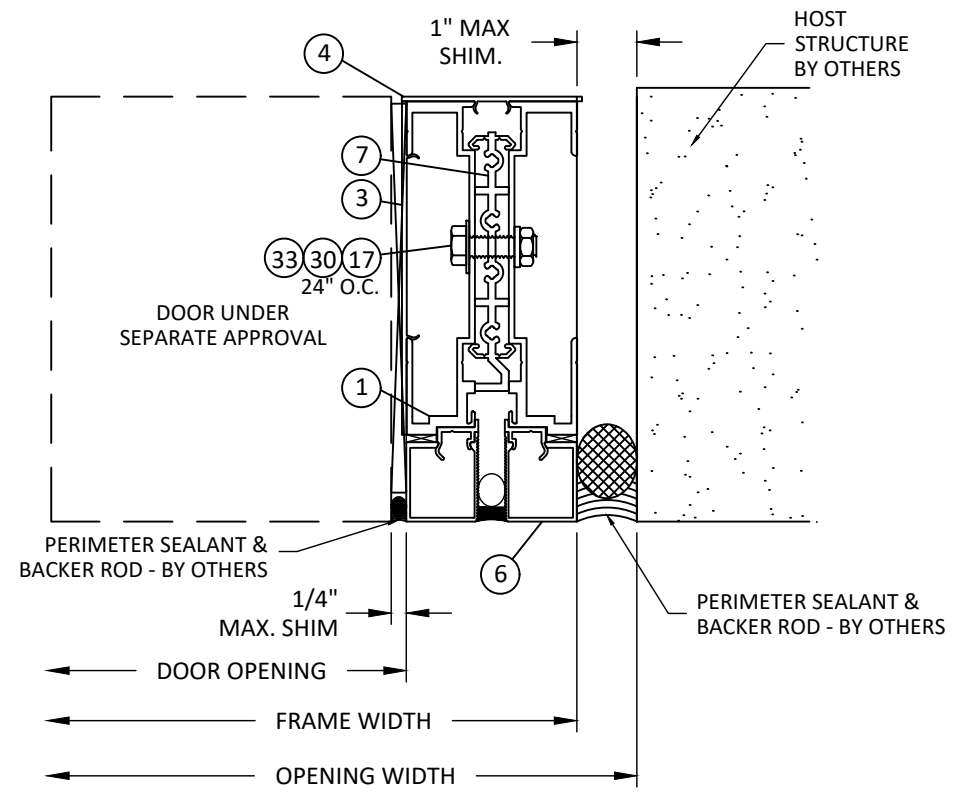
C 6 HORIZONTAL SECTION JAMB - DOOR CONNECTION
