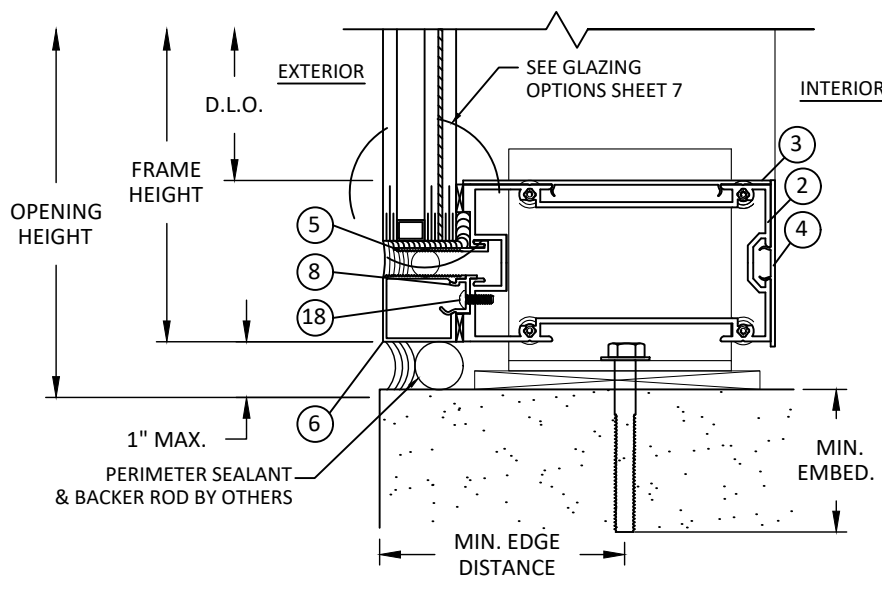
F 3 VERTICAL SECTION SILL - INSULATED GLASS ANCHOR CLIP
