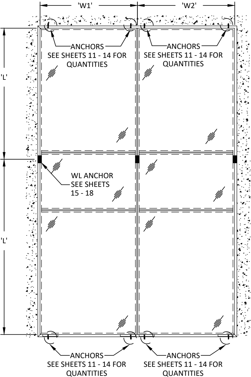
TWIN SPAN ANCHOR LAYOUT
