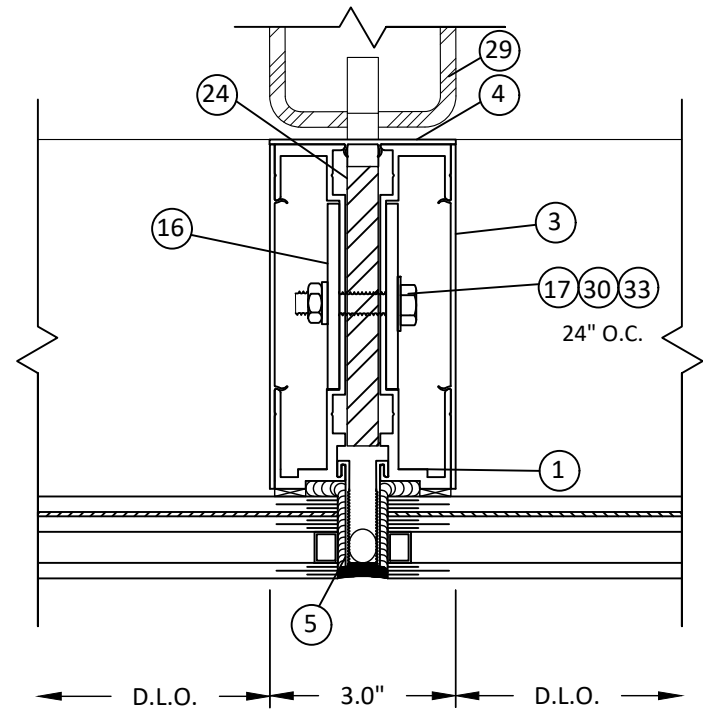
E 4 HORIZONTAL SECTION VERTICAL INTERMEDIATE - INSULATED GLASS TIE BACK ANCHOR AT SPLICE
