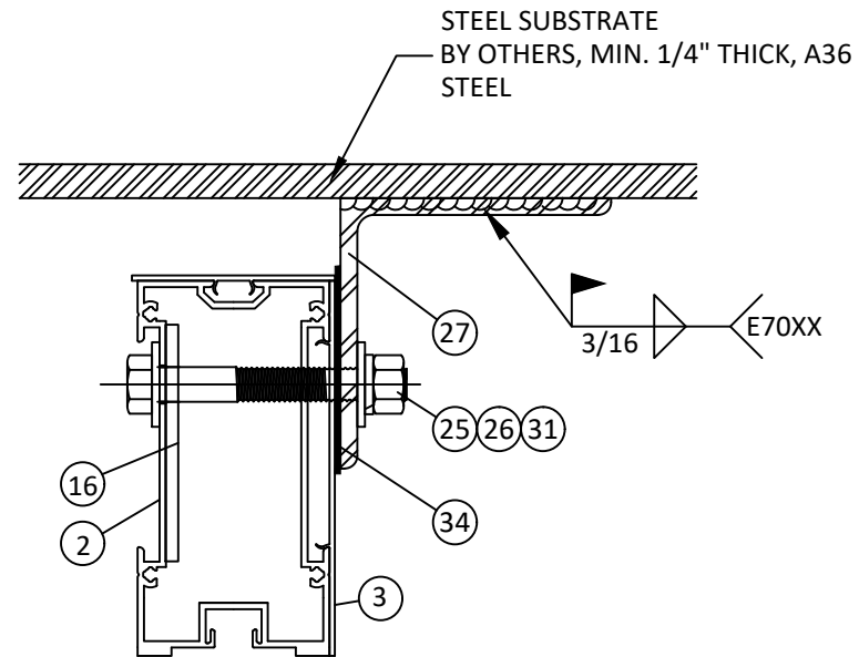
A 15 HORIZONTAL SECTION WIND LOAD ANCHOR AT JAMB
