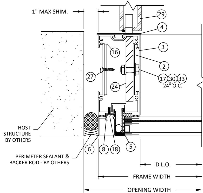
E 5 HORIZONTAL SECTION JAMB - INSULATED GLASS TIE BACK ANCHOR AT SPLICE
