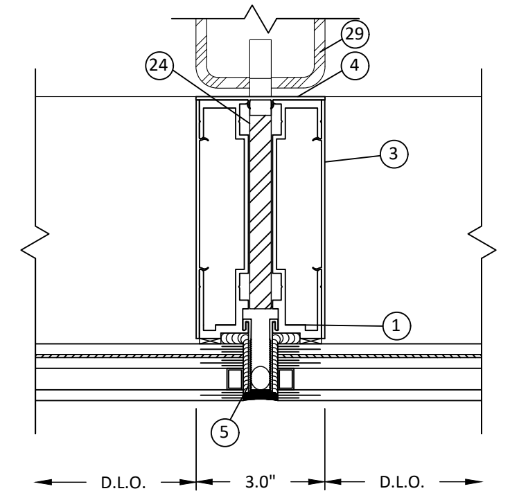
F 4 HORIZONTAL SECTION VERTICAL INTERMEDIATE - INSULATED GLASS TIE BACK ANCHOR ABOVE SPLICE
