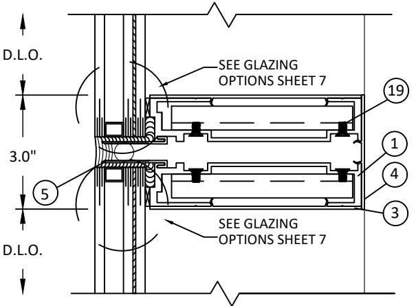
E 3 VERTICAL SECTION HORIZONTAL PANEL TO PANEL MULLION - INSULATED GLASS EXPANSION HORIZONTAL CONDITION
