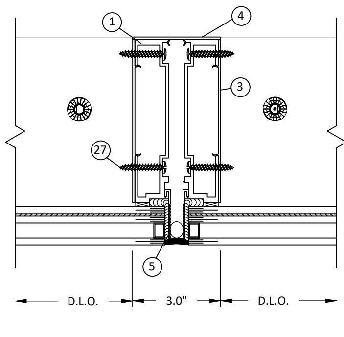
A 6 HORIZONTAL SECTION INTEGRATED VERTICAL INTERMEDIATE - INSULATED GLASS ANCHORS THROUGH SILL
