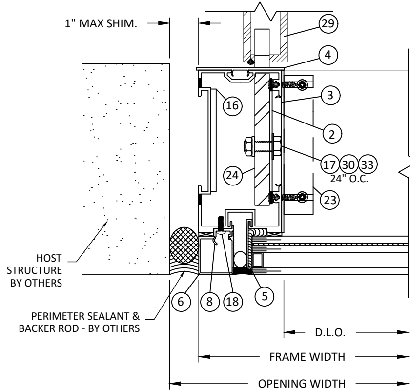
D 5 HORIZONTAL SECTION JAMB - INSULATED GLASS TIE BACK ANCHOR AT PANEL TO PANEL CONNECTION
