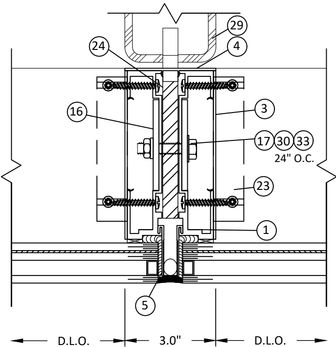
D 4 HORIZONTAL SECTION VERTICAL INTERMEDIATE - INSULATED GLASS TIE BACK ANCHOR AT PANEL TO PANEL CONNECTION
