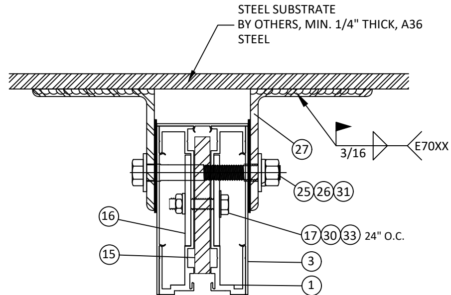
B 15 HORIZONTAL SECTION WIND LOAD ANCHOR AT VERTICAL MULLION
