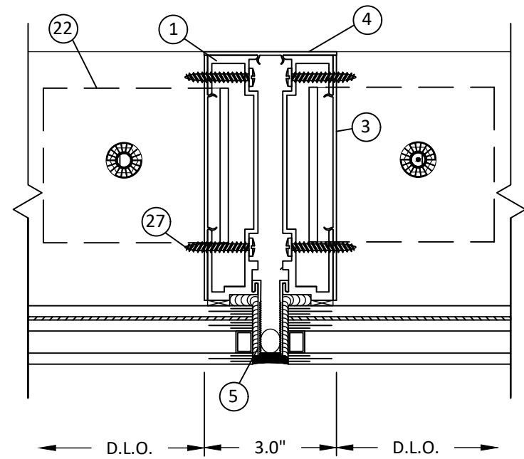
C 4 HORIZONTAL SECTION INTEGRATED VERTICAL INTERMEDIATE - INSULATED GLASS ANCHOR CLIPS
