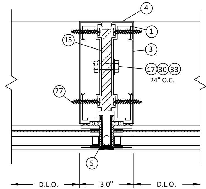
B 4 HORIZONTAL SECTION INTEGRATED VERTICAL INTERMEDIATE - INSULATED GLASS
